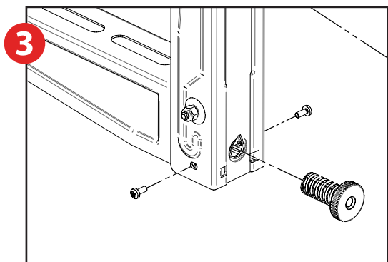
Adjust the distance of the arms to the wall using the nylon screws.
