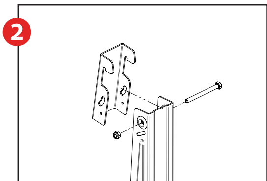
Using the appropriate nuts and bolts, secure the hooks to the upper arms.
