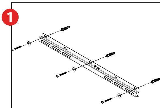
Level and fix the supplied crossbar to the wall. Use plugs at your discretion.
