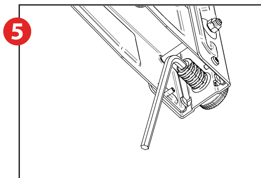
Fasten dampers at the corner with flat side facing the back.
