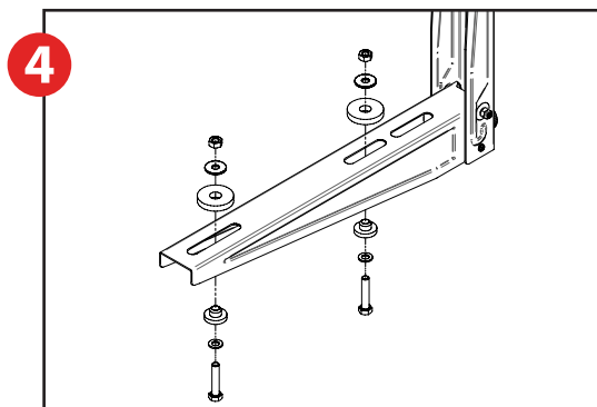
Place the washers on the horizontal arms.
